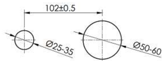
Mounting Hole
