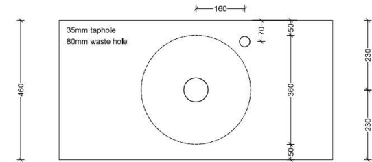
Taphole Offset
