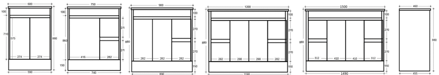
1200mm - #K-PF1200
