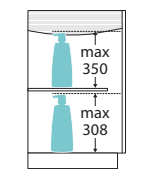
SIDE VIEW: SHELF STORAGE
