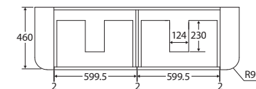
SIDE VIEW: DRAWER STORAGE
