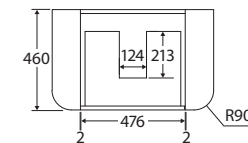
SIDE VIEW: DRAWER STORAGE
