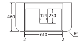
SIDE VIEW: DRAWER STORAGE
