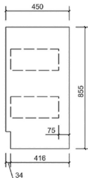
End view
